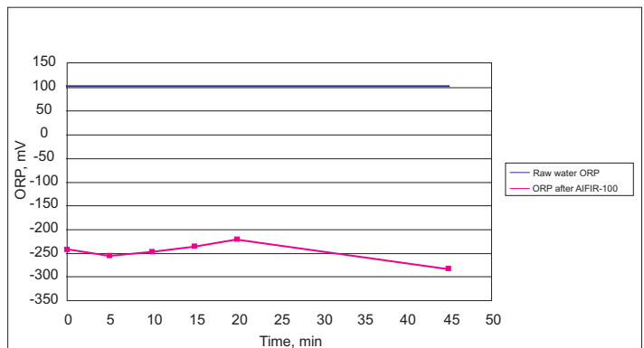
ORP of water RO after passing through AIFIR-100
