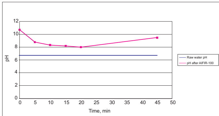
pH of water RO after passing through AIFIR-100
