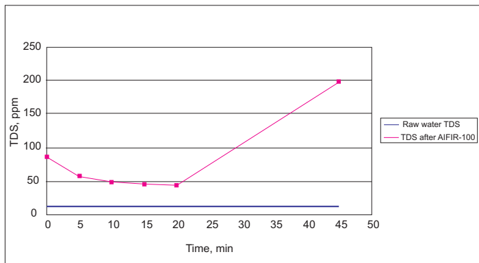
TDS of RO water after passing through AIFIR-100
